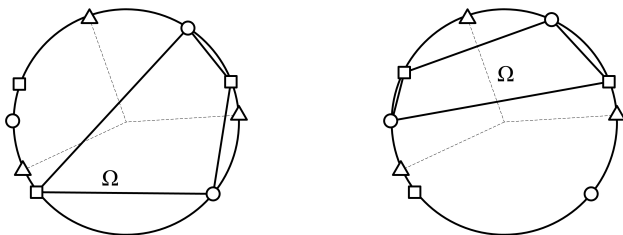
FIGURE 1. Two-dimensional cross-polytopes \Omega containing \mathbf{0} and not.
