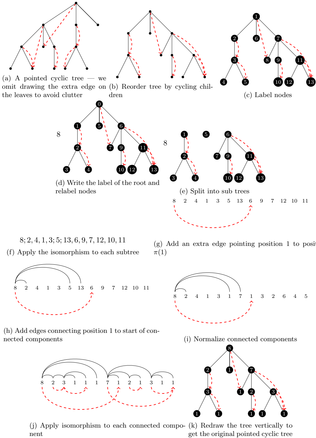
Figure 2.3.11: An example of the isomorphism from pointed cyclic trees to connected permutations. (b)–(f) is the isomorphism and (g)–(k) is the inverse isomorphism.
