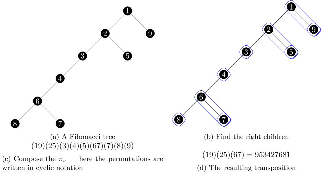
Figure 2.3.2: An example of the isomorphism from increasing Fibonacci trees to involutions. Note that reading off the labels of the tree in infix order gives the permutation 867432519 that is not an involution.
