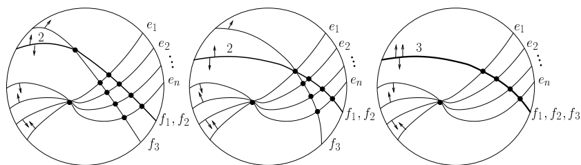
FIG. 3. Three wiring diagrams with alternating orientations.
