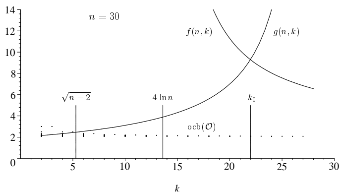
FIG. 5. f(n, k) , g(n, k) , and \text{ocb}(\mathcal{O}) versus k , when n = 30 .
