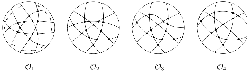
FIG. 2. The four reclasses of the uniform matroid U_{3,6} .
