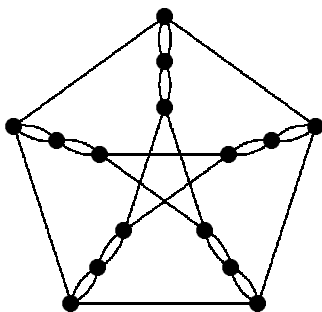
Figure 1 A 2-connected 4-regular eulerian graph without removable circuit.
