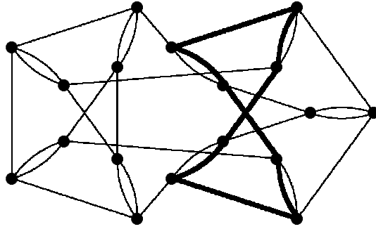
Figure 3 A 2-connected graph containing no circuit decomposition in which all circuits have length at least 3, but containing a removable circuit (shown in bold) of length at least 3.
