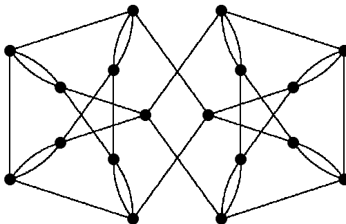
Figure 2 A 2-connected graph containing circuit decompositions in which every circuit has length at least 3, but containing no removable circuit of length at least 3.
