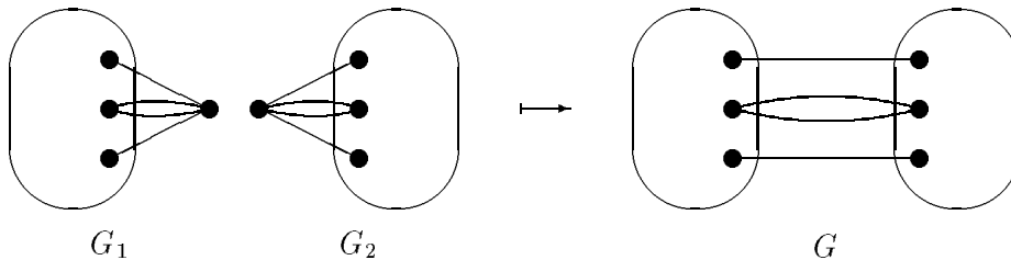
Figure 5 If neither G_1 nor G_2 has a removable circuit different from a lonely digon, then neither has G .
