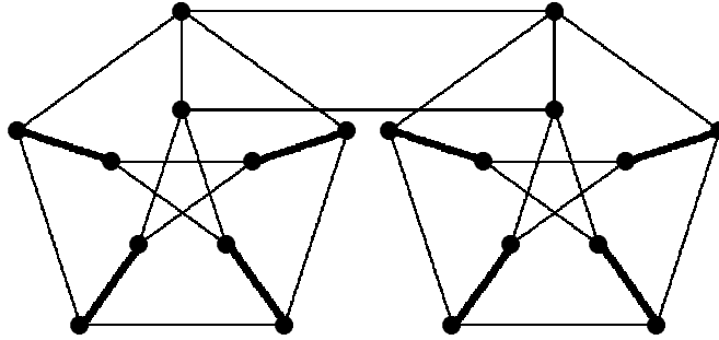
Figure 4 A 2-connected edge-weighted graph ( thin edges have weight 1, bold edges have weight 2 ) having a faithful circuit cover, but no faithful circuit cover that satisfies the properties in Lemma 4.2.
