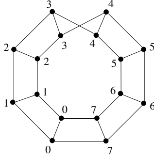
Figure 3: A Möbius ladder of order 16.
