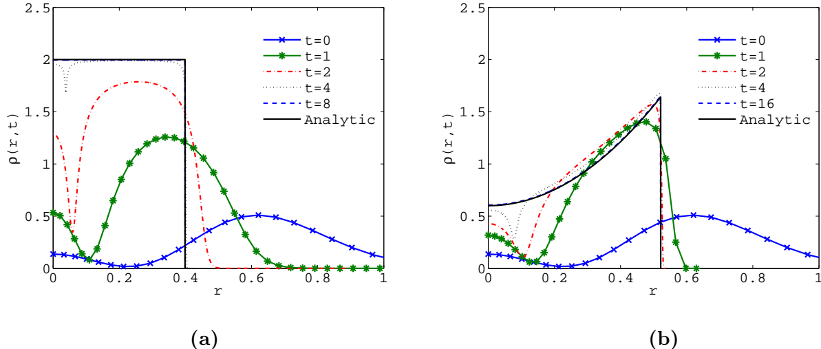
Figure 3: Time evolution of a radially symmetric solution to the aggregation model (1), (8) with (a) q = 2 and (b) q = 4 , in two dimensions, starting from initial data (69). (a) As predicted by the analytical results from Section 2, the solution approaches asymptotically a constant, compactly supported steady state. (b) The solution approaches asymptotically the steady state computed analytically in Section 3.2 — see equations (61), (63) and (64).
