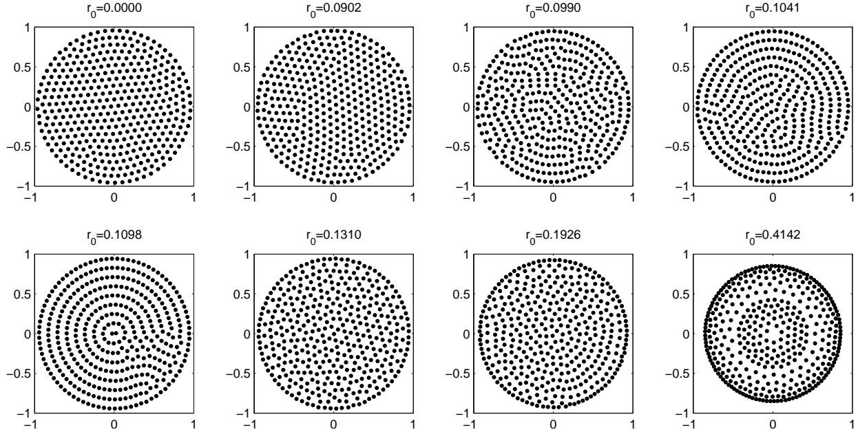
Figure 6: Equilibrium states for the truncated interaction force (94) with N = 400 . The equilibrium is computed by integrating the ODE system (5) to t = 5000 , starting from random initial conditions in the unit square. For r_0 < 0.09 , the steady state is the same as for r_0 = 0 (uniform density in the unit circle). As r_0 is increased further, intricate grid defects are observed, while the overall swarm radius and density remain roughly the same. Finally, for r_0 > 0.2 , the uniformity of the swarm breaks down leading to a very different steady state.
