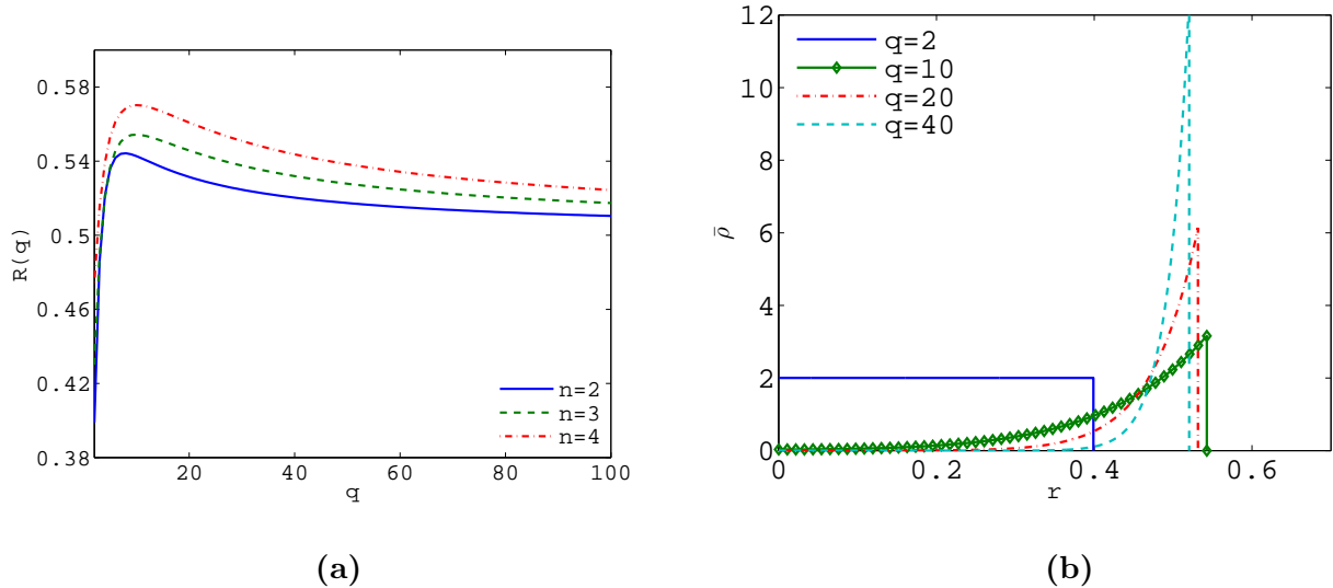
Figure 2: (a) Plot of the radius of the support R of the steady states of (1), (8), as a function of the exponent q , for various space dimensions n . The plot suggests that the radius R approaches asymptotically a constant, as q \rightarrow \infty . (b) Normalized radially symmetric steady states \bar{\rho}(r) of (1), (8) in two dimensions for various values of the exponent q . For q = 2 the steady state is the constant solution in a disk. As q increases, the qualitative features of the steady states change, as mass aggregates toward the edge of the swarm, creating an increasingly void region in the centre. This suggests that, as q \rightarrow \infty , the steady states in two dimensions approach a ring solution of non-zero radius.
