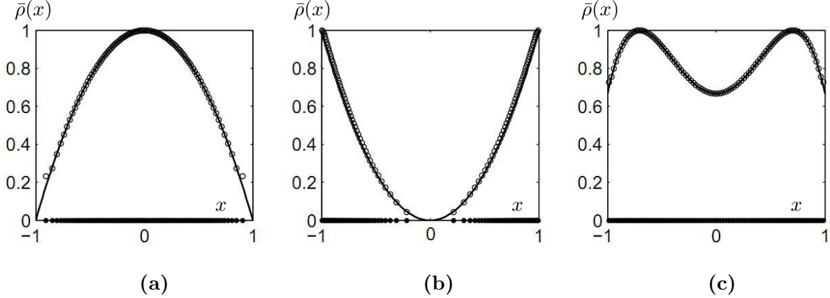
Figure 4: (a)-(c) Steady state solutions to (1) in one dimension with force F(x) given by (77). Filled circles along the x-axis represent the steady state for the corresponding dynamical system (5) with N = 50 particles. Empty circles represent the density function as computed from the filled circles, normalized so that \max \bar{\rho} = 1 . The solid line is the analytical expression for \bar{\rho} given by (76), but normalized so that \max \bar{\rho} = 1 . In all cases, excellent agreement is observed between the asymptotic behaviour and the predicted steady states.
