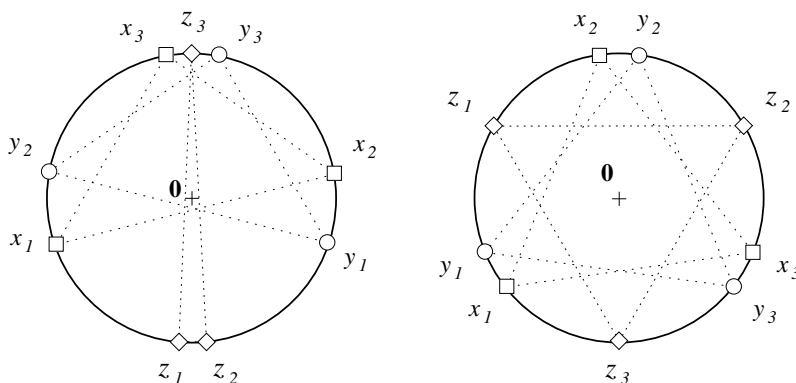
FIGURE 5. The two configurations in dimension 2 with \mathbf{depth}_{\mathbf{S}}(\mathbf{0}) = 9 .
