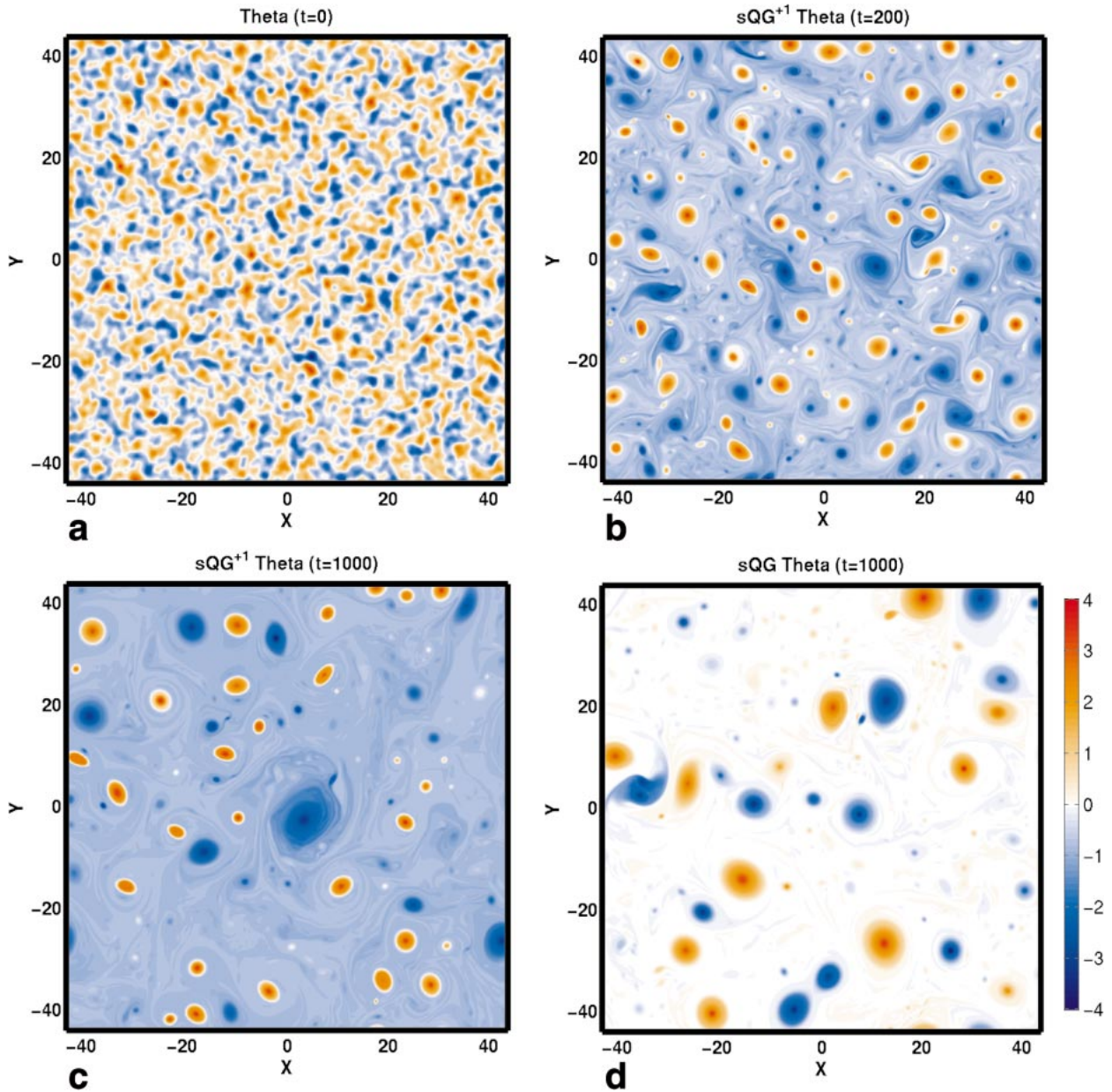
FIG. 1. Surface potential temperature evolution for numerical solutions of sQG^{+1} [panels (b) and (c)] and sQG [panel (d)] freely decaying turbulence. The random initial condition shown in (a) evolves into a field of vortices and filaments by t = 200 (b). By t = 1000 , cyclone-anticyclone asymmetries and surface cooling are prominent in the sQG^{+1} solution (c) and are absent in the sQG solution (d). All units are nondimensional, and the Rossby number ( \epsilon ) is 0.1 for the sQG^{+1} solution.
