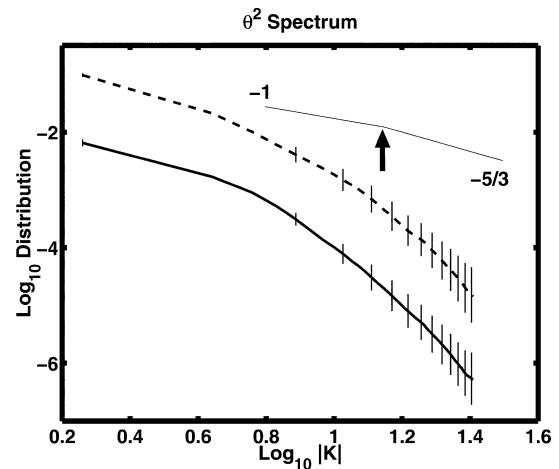
FIG. 3. Ensemble-mean surface potential temperature variance spectra. The sQG curve (dashed line) has been displaced from the sQG +1 curve (solid line) for clarity. Thin vertical lines show \pm 1 ensemble standard deviation around the ensemble mean, and lines with slopes of -5/3 and -1 are provided for reference. The spectral peak in the initial condition is denoted by the bold arrow.
