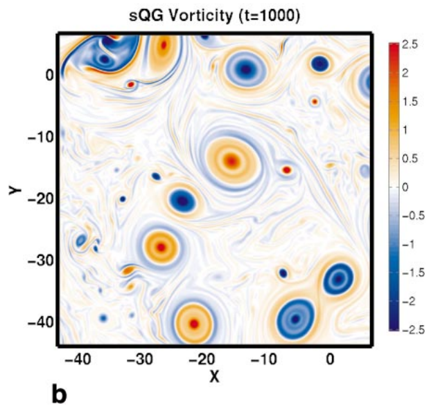
FIG. 10. Vertical component of relative vorticity at t = 1000 for (a) sQG^{+1} and (b) sQG solutions. The vorticity shown in (b) is leading-order only, whereas in (a) the vorticity is correct to O(\epsilon) . Here, (a) corresponds to the upper left quadrant of Fig. 1c, and (b) corresponds to the lower left quadrant of Fig. 1d.
