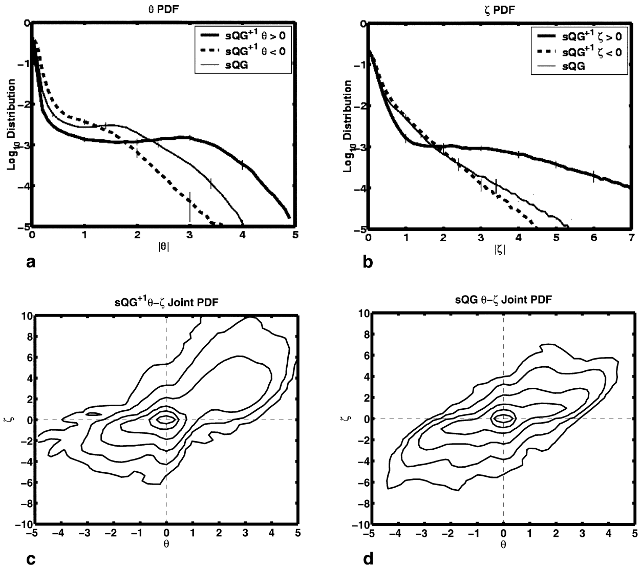
FIG. 5. Ensemble-mean PDFs for (a) surface potential temperature \theta^* - \bar{\theta}^* , and (b) vorticity and joint PDFs of surface potential temperature \theta^* - \bar{\theta}^* , and vorticity for (c) \text{sQG}^{+1} and (d) \text{sQG} . In (a) and (b), values for \theta^* - \bar{\theta}^* < 0 have been folded across the origin, with positive values given by thick solid lines and negative values given by thick dashed lines; the symmetric \text{sQG} curve is given by a thin solid line. Thin vertical lines show \pm 1 ensemble standard deviation around the ensemble mean. Contours in (c) and (d) are given in powers of 10, with an innermost contour of 0.1.
