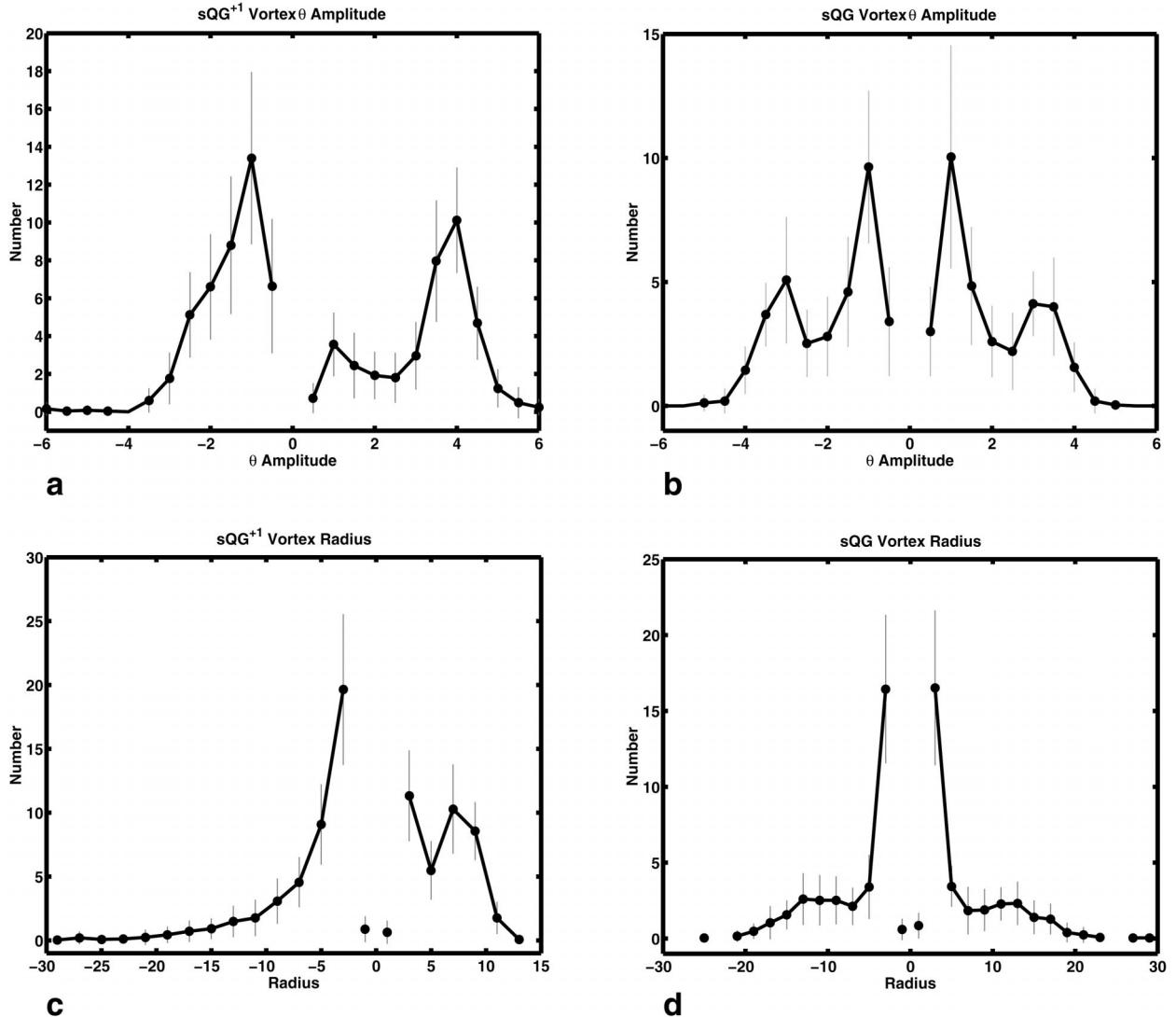
FIG. 6. Vortex census data at t = 1000 showing (a), (b) ensemble-mean vortex amplitude and (c), (d) radius; note that vortex amplitude is defined relative to \bar{\theta} . The sQG + solutions are given in (a) and (c), and the sQG solutions are given in (b) and (d). Thin vertical lines show \pm 1 ensemble standard deviation around the ensemble mean, which is given by the bold solid line.
