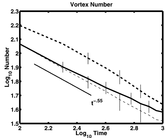
FIG. 8. Vortex number as a function of time. The thin dashed line represents sQG vortices, the thick solid line represents sQG + cyclones, and the thick dashed line represents sQG + anticyclones. A solid line with slope -0.55 is provided for reference.
