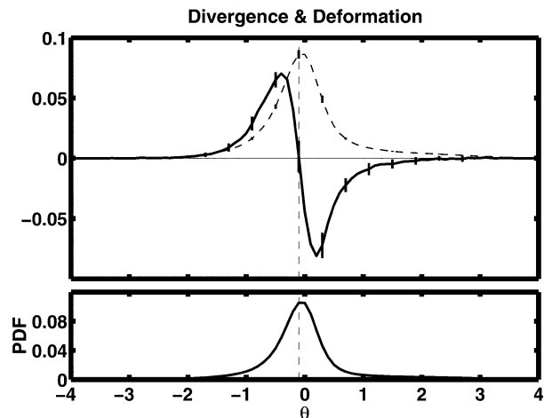
FIG. 4. Average surface divergence (solid line) and deformation (dashed line) at t = 1000 as a function of perturbation surface potential temperature \theta^s - \bar{\theta}^s (upper panel). These ensemble-mean curves represent averages over grid points for \theta^s - \bar{\theta}^s within \pm 0.05 of the central value given on the abscissa. The ensemble-mean PDF for \theta^s - \bar{\theta}^s at t = 1000 is shown in the lower panel. Thin solid vertical lines show \pm 1 ensemble standard deviation around the ensemble mean, and the thin dashed vertical line denotes the peak of the \theta^s - \bar{\theta}^s PDF; note that this is a skewed distribution.
