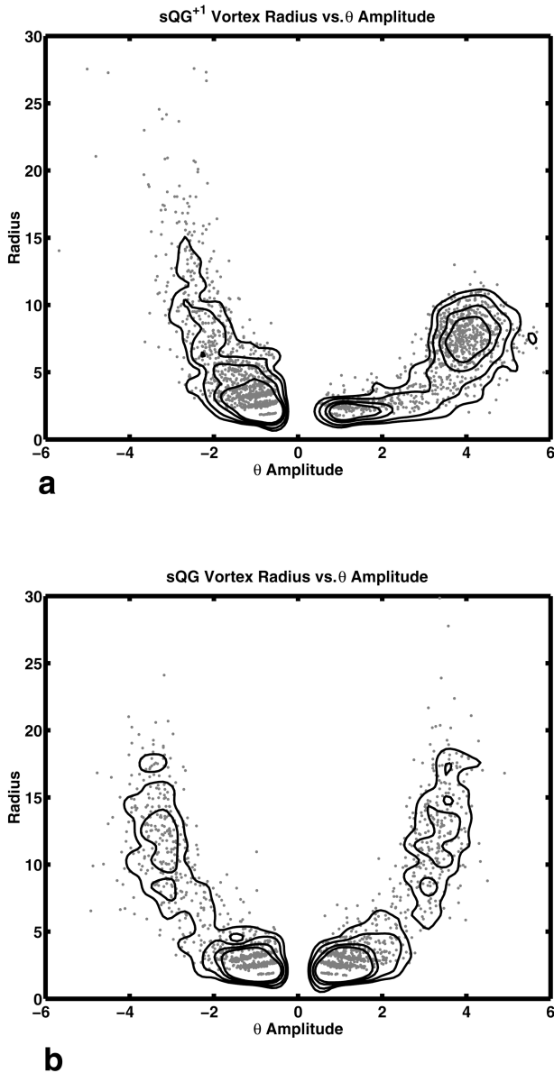
FIG. 7. Vortex radius as a function of amplitude \theta^s - \bar{\theta}^s for (a) sQG + and (b) sQG solutions at t = 1000 . Each vortex is represented by a dot, and the solid lines are constant-density contours (0.005, 0.01, 0.02, 0.03) of the joint PDF.
