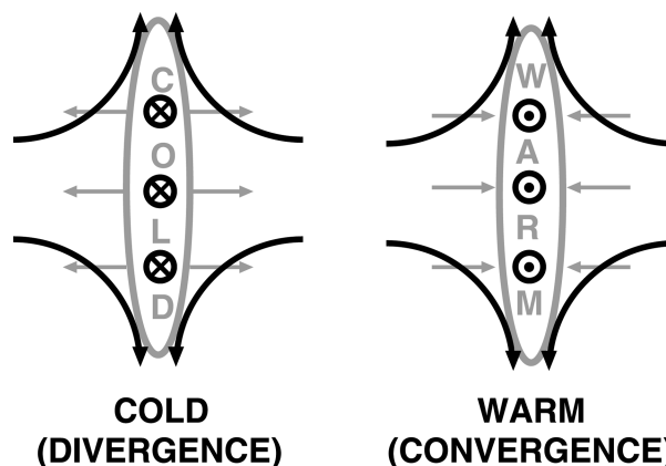
FIG. 11. Schematic illustration of the divergent-flow response to (a) cold and (b) warm filaments in deformation. Black arrows show the ambient deformation that acts to thin the filaments (thick gray lines) and provoke the divergent response in the vertical plane normal to the filaments (arrow heads and arrow tails). The net affect of the divergent motions, given by the gray arrows, is to accelerate the contraction of warm filaments relative to cold filaments.
