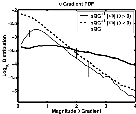
FIG. 9. The t = 1000 ensemble-mean PDFs for magnitude of the horizontal gradient of surface potential temperature, conditioned on |\theta^* - \bar{\theta}^*| > 1 . Cyclonic sQG^{+1} (positive) values are given by thick solid lines, and anticyclonic sQG^{+1} (negative) values are given by thick dashed lines; the symmetric sQG curve is given by a thin solid line. Short vertical lines show \pm 1 ensemble standard deviation around the ensemble mean.
