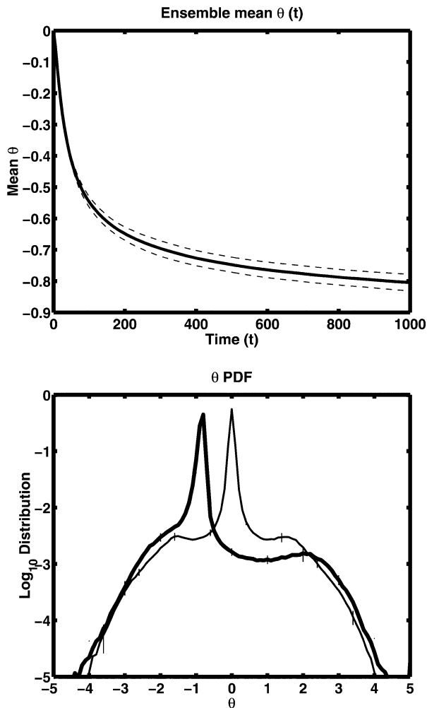
FIG. 2. (a) Mean surface potential temperature \bar{\theta} as a function of nondimensional time. Dashed lines show \pm 1 ensemble standard deviation about the ensemble mean (bold line). (b) Potential temperature PDF at t = 1000 for sQG +1 (thick line) and sQG (thin line). Vertical lines show \pm 1 ensemble standard deviation around the ensemble mean.
