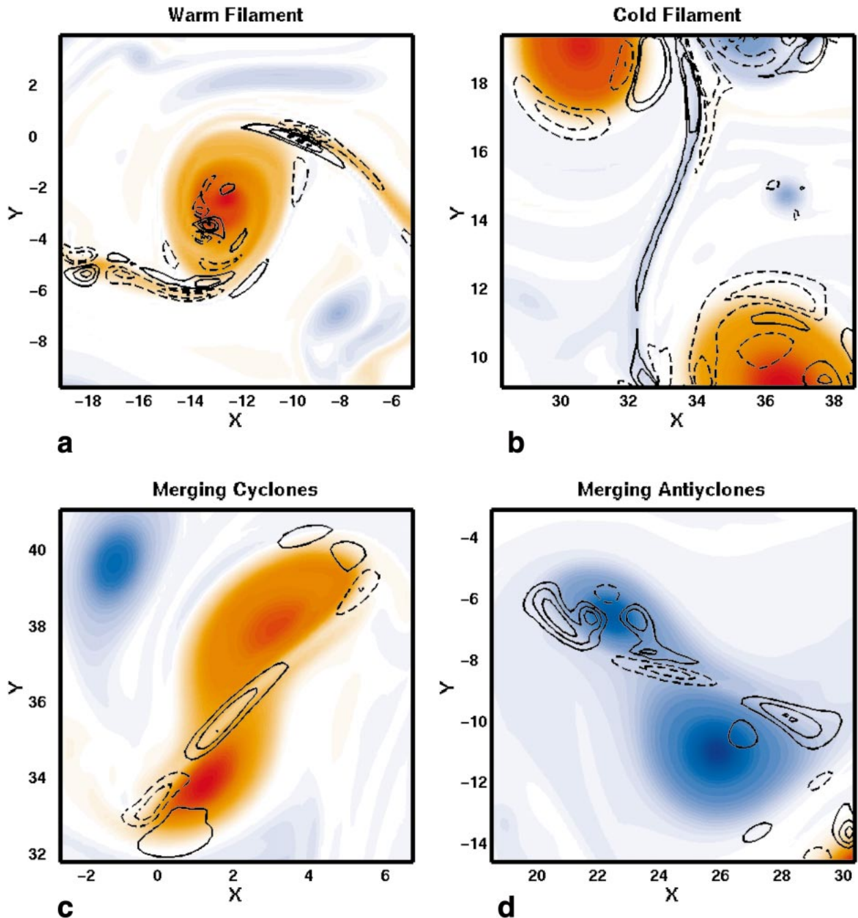
FIG. 12. Surface potential temperature (colors) and divergence (black lines) for examples of (a) warm filaments, (b) cold filaments, (c) merging cyclones, and (d) merging anticyclones. Solid lines show divergence, and dashed lines show convergence.
