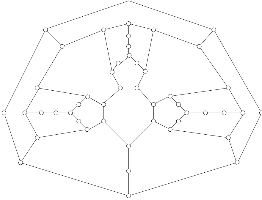
Figure 1: Albertson-Moore graph
