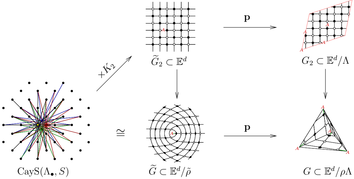
Figure 3: Constructing finite Cayley sum graph from a lattice. Illustrated with the D_2 -lattice, resulting in a 28-vertex Cayley sum graph which is also a 4-regular quadrangulation of the tetrahedron.
